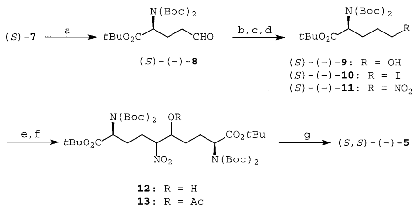
Scheme 2. Synthesis of (S,S) -(-)-5. Reagents and conditions: a) See ref. [17]; b) NaBH_4 (1.0 equiv), MeOH, 0 °C, 45 min, 95%; c) I_2 (1.5 equiv), PPh_3 (1.6 equiv), imidazole (2.0 equiv), THF, 23 °C, 1.5 h, 94%; d) NaNO_2 (2.0 equiv), DMF, 23 °C, 30 min, 55%; e) (S) -(-)-8 (1.1 equiv), DMAP, (4.0 equiv), CH_2Cl_2 , 23 °C, 8 d, 91%; f) Ac_2O (1.5 equiv), DMAP (0.1 equiv), THF, 23 °C, 2 h, 96%; g) BnO_2CCH_2NC ( 14 , 1.3 equiv), DBU (2.5 equiv), THF, 0–23 °C, 5 h, 57%. DBU = 1,8-diazabicyclo[5.4.0]undec-7-ene, DMAP = 4-dimethylaminopyridine.
